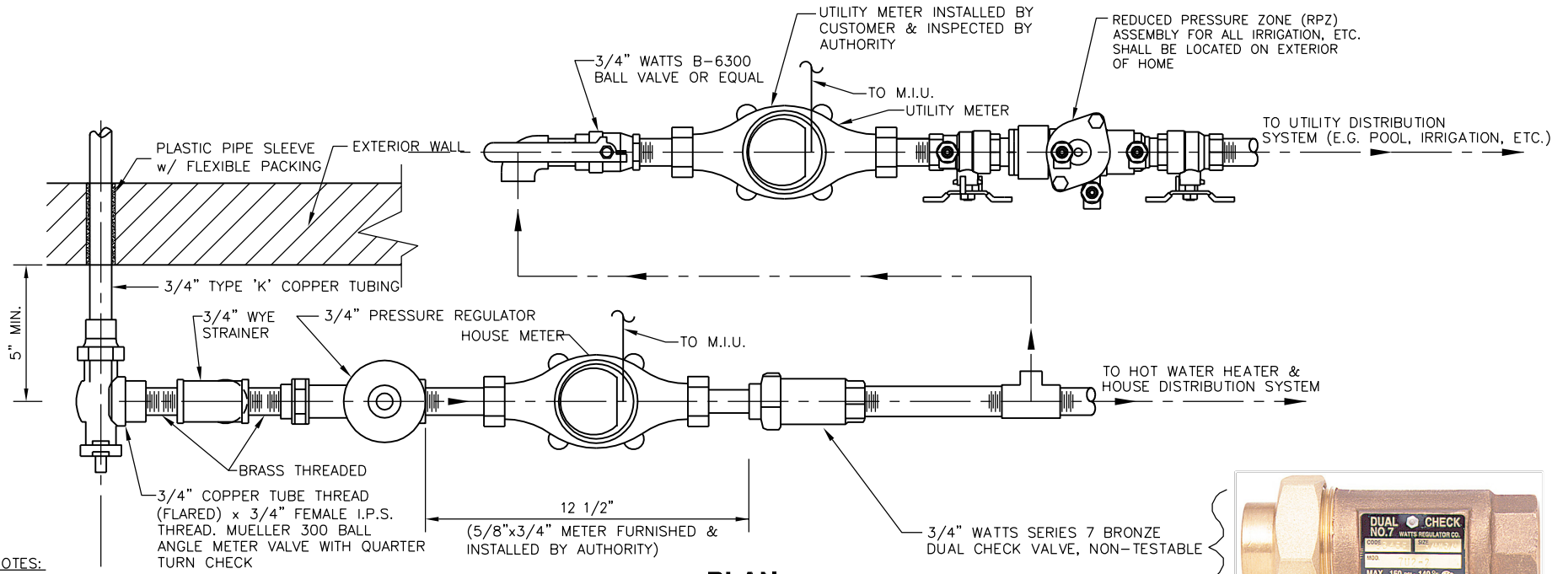
PLAN
